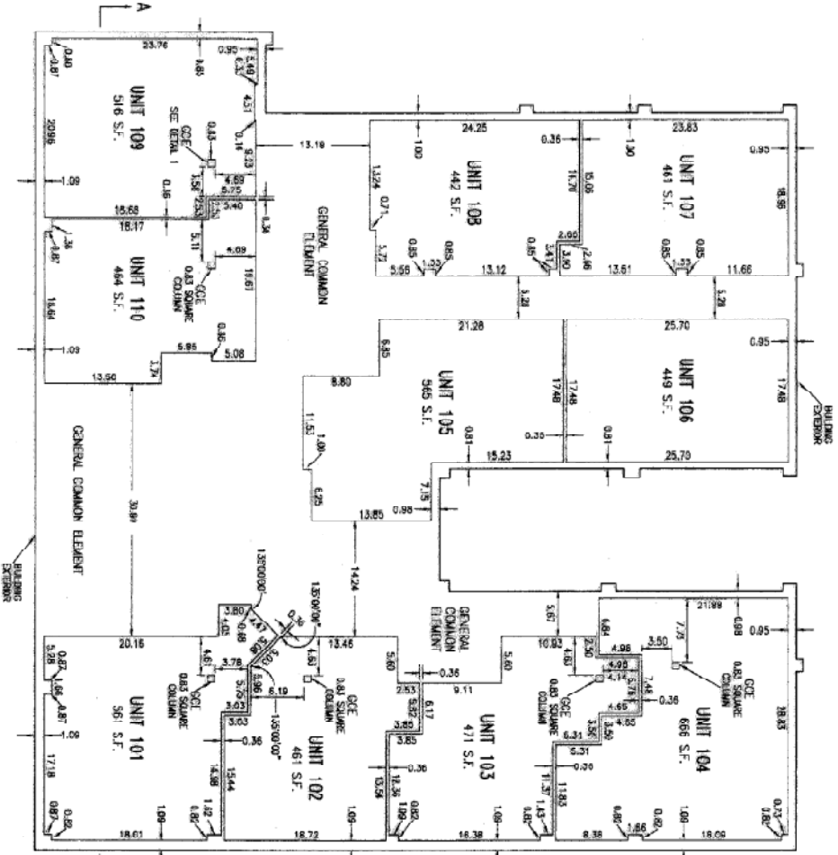
FIRST FLOOR PLAN SCALE: 1"=10'
